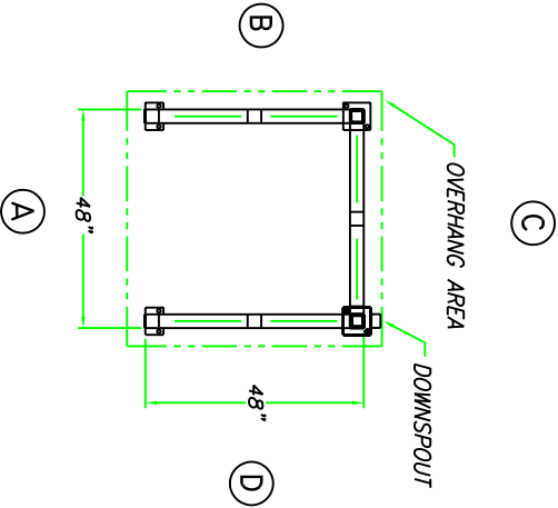
PLAN VIEW SCALE: 1/2"=1'
