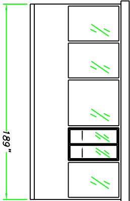
ELEVATION C
