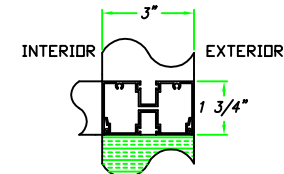
VIEW C-C
