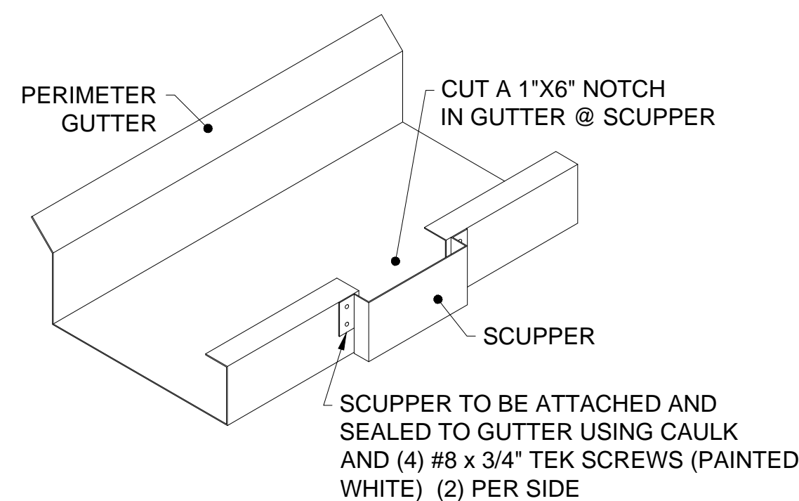
SCUPPER DETAIL
