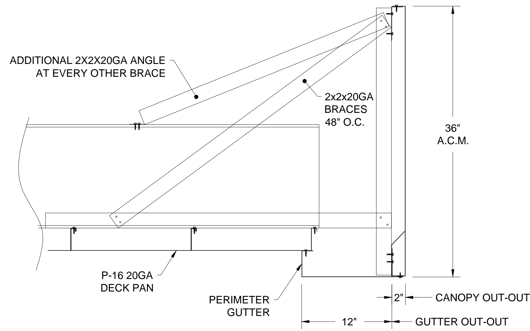
DETAIL A: 36'-0" SIDE FASCIA BRACE DETAIL
