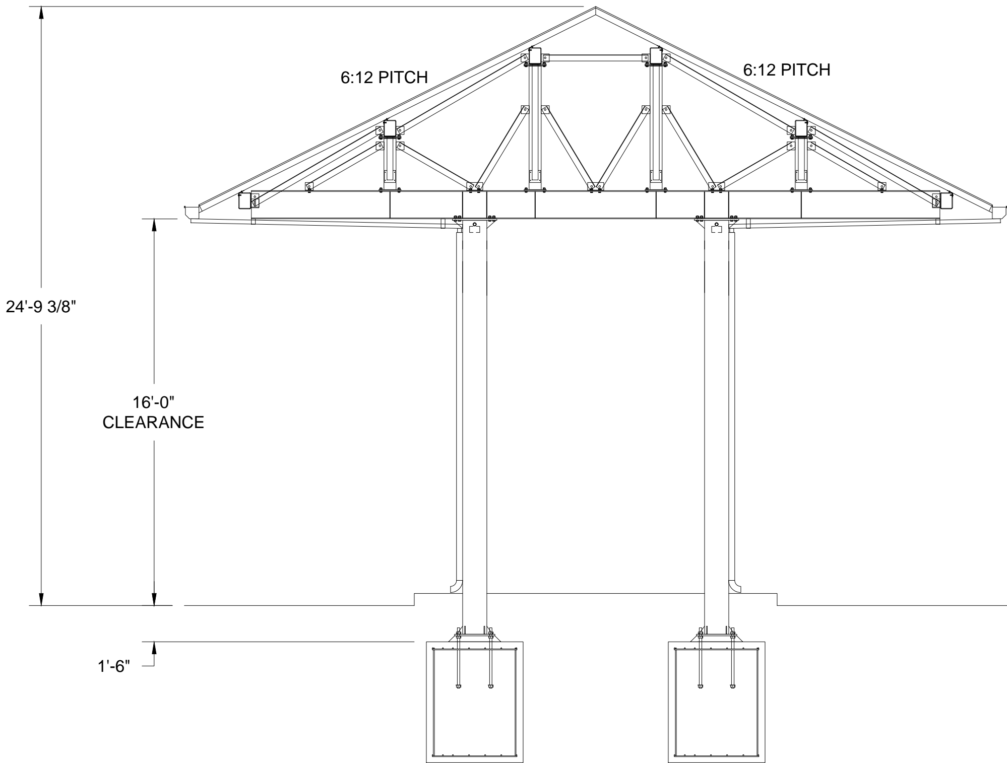
END VIEW
