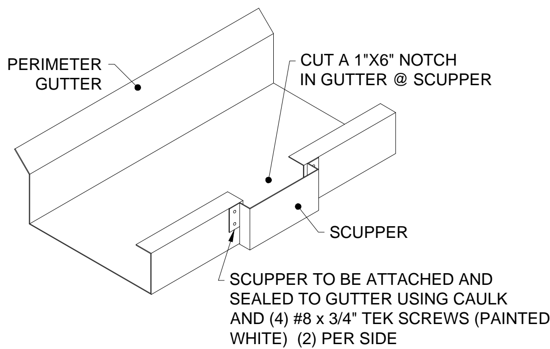
SCUPPER DETAIL
