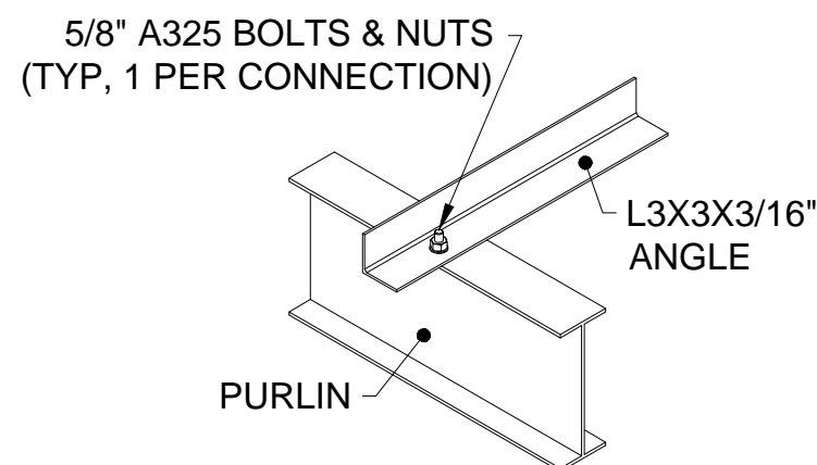
ANGLE BRACE DETAIL
