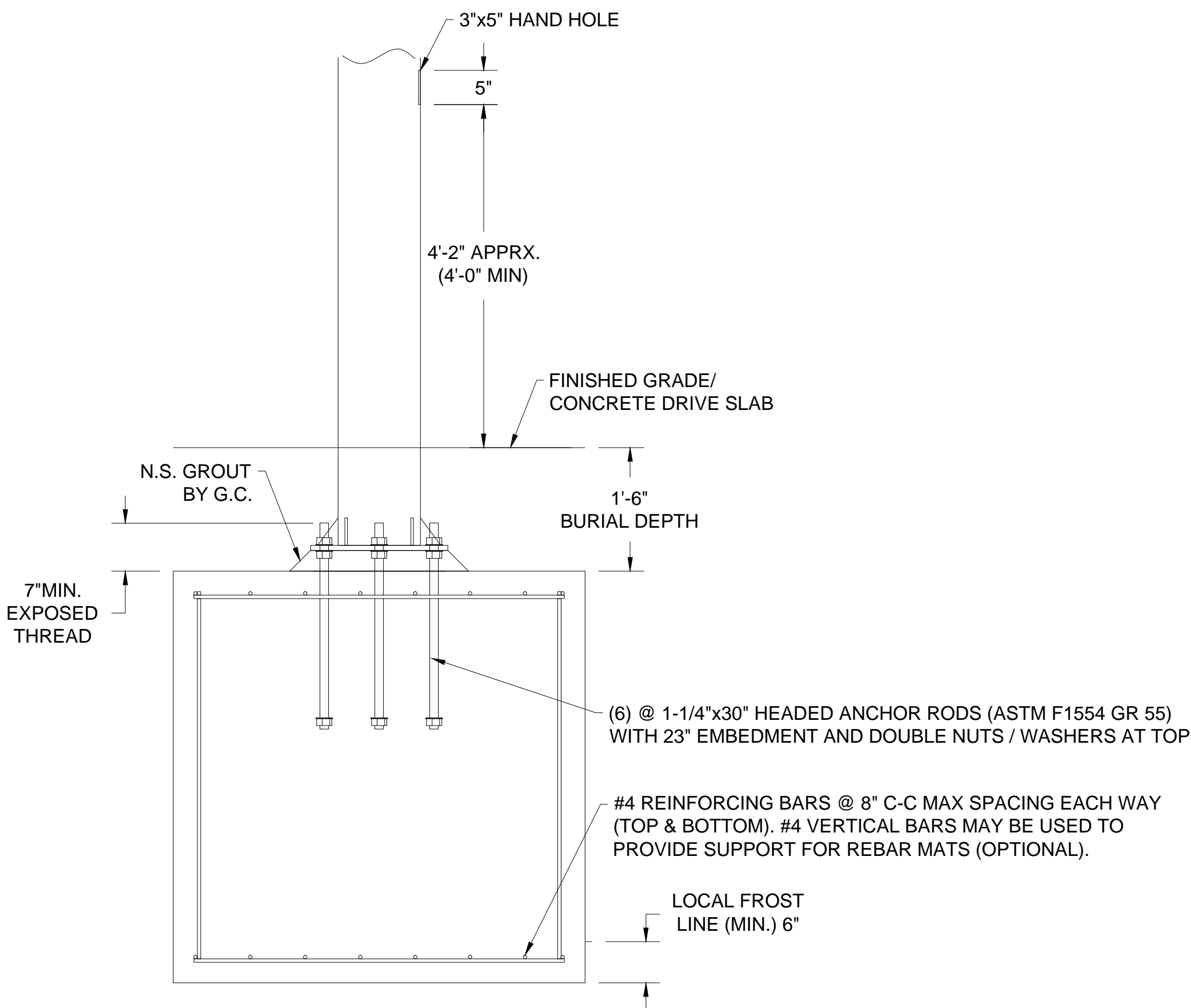
SECTION C-C
